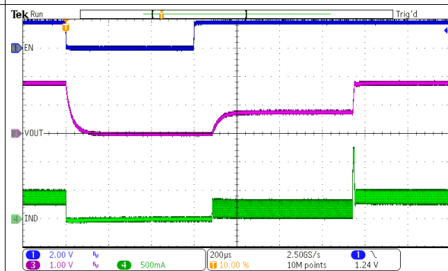
Figure 53. 100% Mode Entry/Exit Operation
